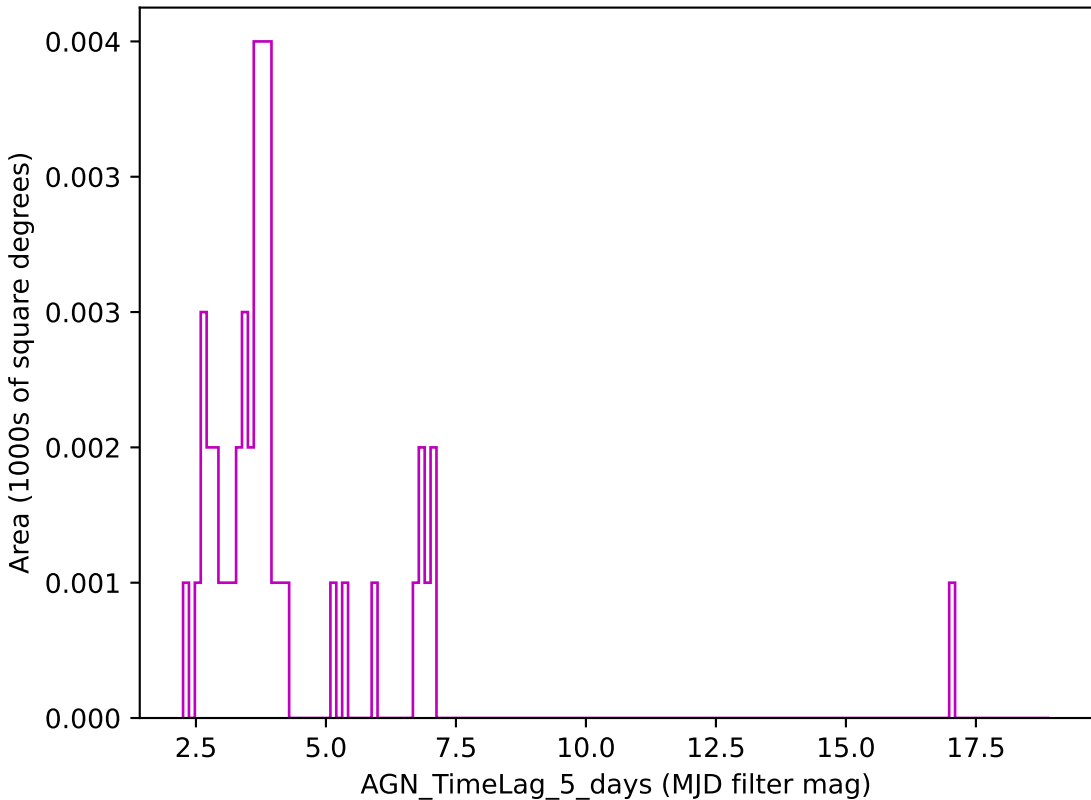
too_elab_r256_d3_griz_v3.4_10yrs z band: AGN_TimeLag_5_days
