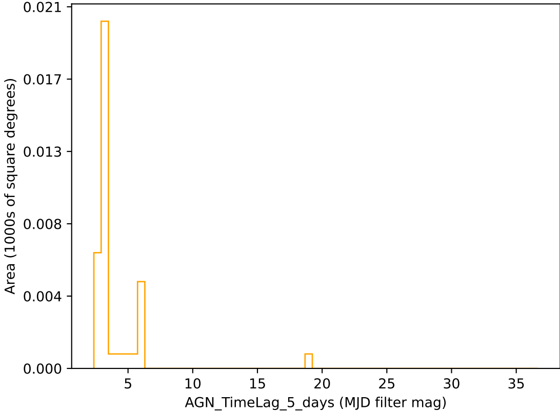
too_elab_r256_d3_griz_v3.4_10yrs r band: AGN_TimeLag_5_days
