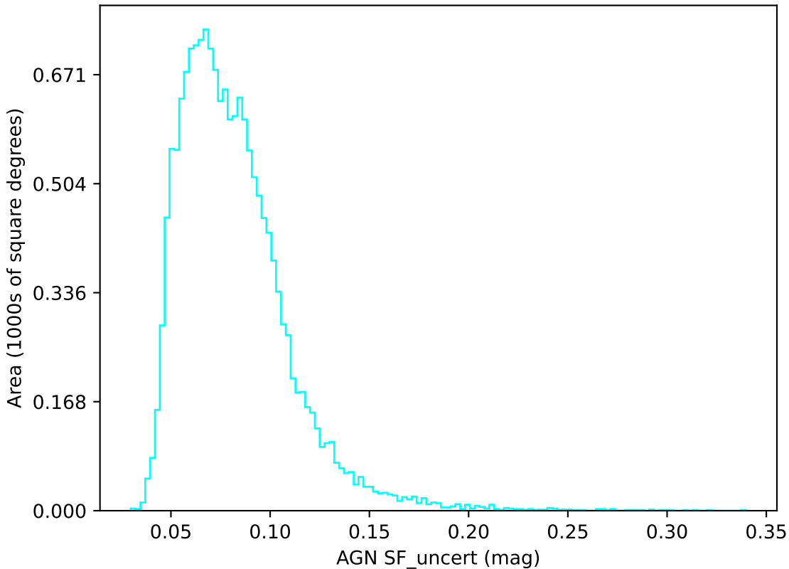
too_elab_r256_d3_griz_v3.4_10yrs u band: AGN SF_uncert
