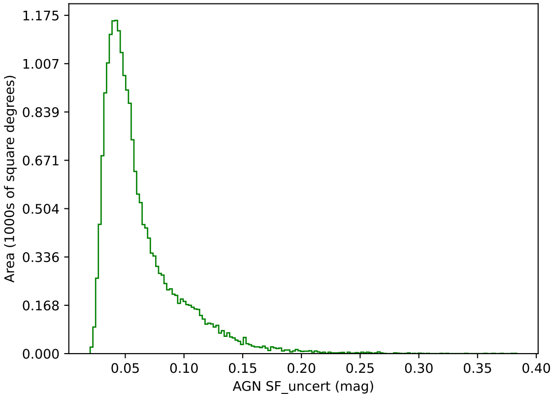
too_elab_r256_d3_griz_v3.4_10yrs g band: AGN SF_uncert
