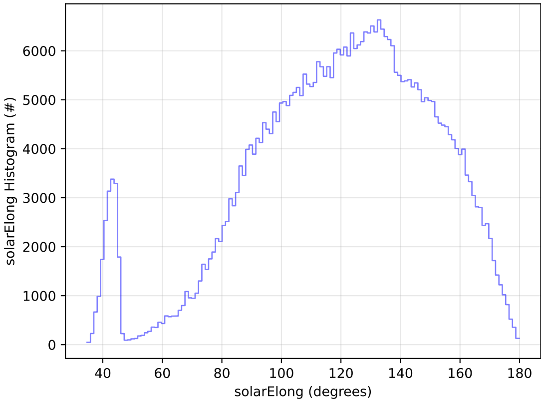
too_elab_r256_d3_griz_v3.4_10yrs WFD z band: solarElong Histogram
