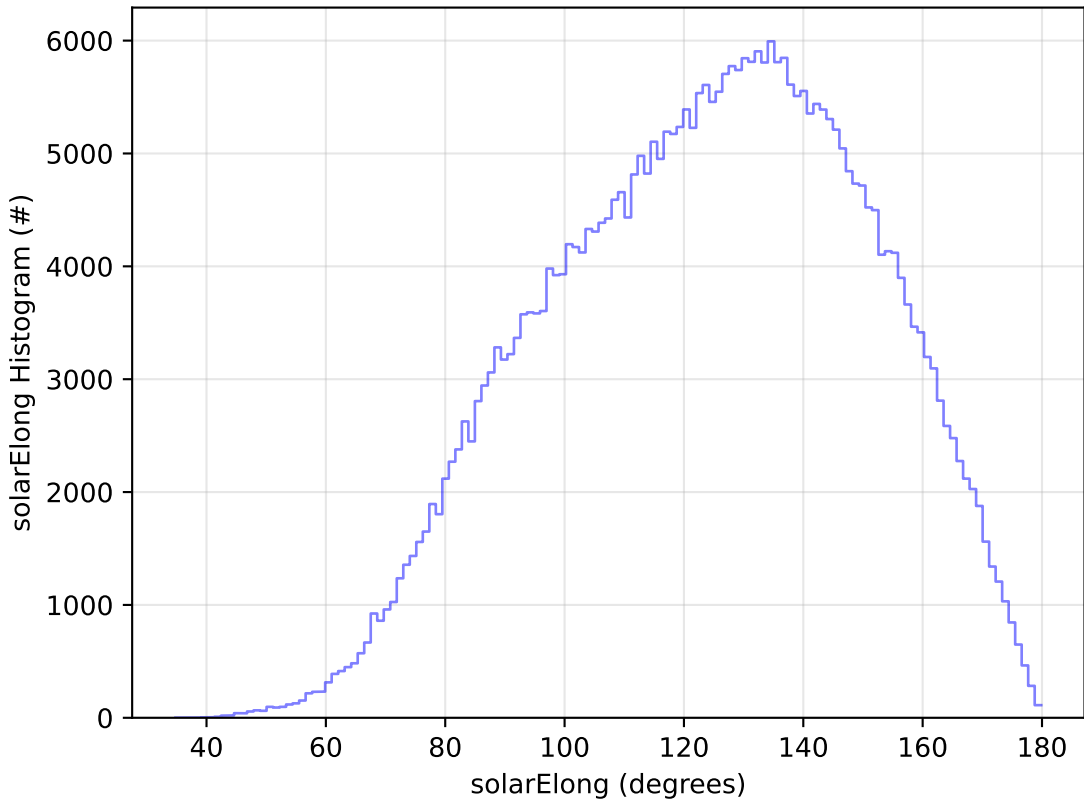
too_elab_r256_d3_griz_v3.4_10yrs WFD y band: solarElong Histogram
