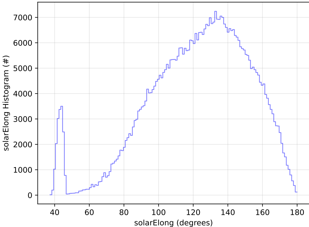
too_elab_r256_d3_griz_v3.4_10yrs WFD r band: solarElong Histogram
