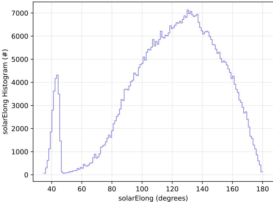
too_elab_r256_d3_griz_v3.4_10yrs WFD i band: solarElong Histogram
