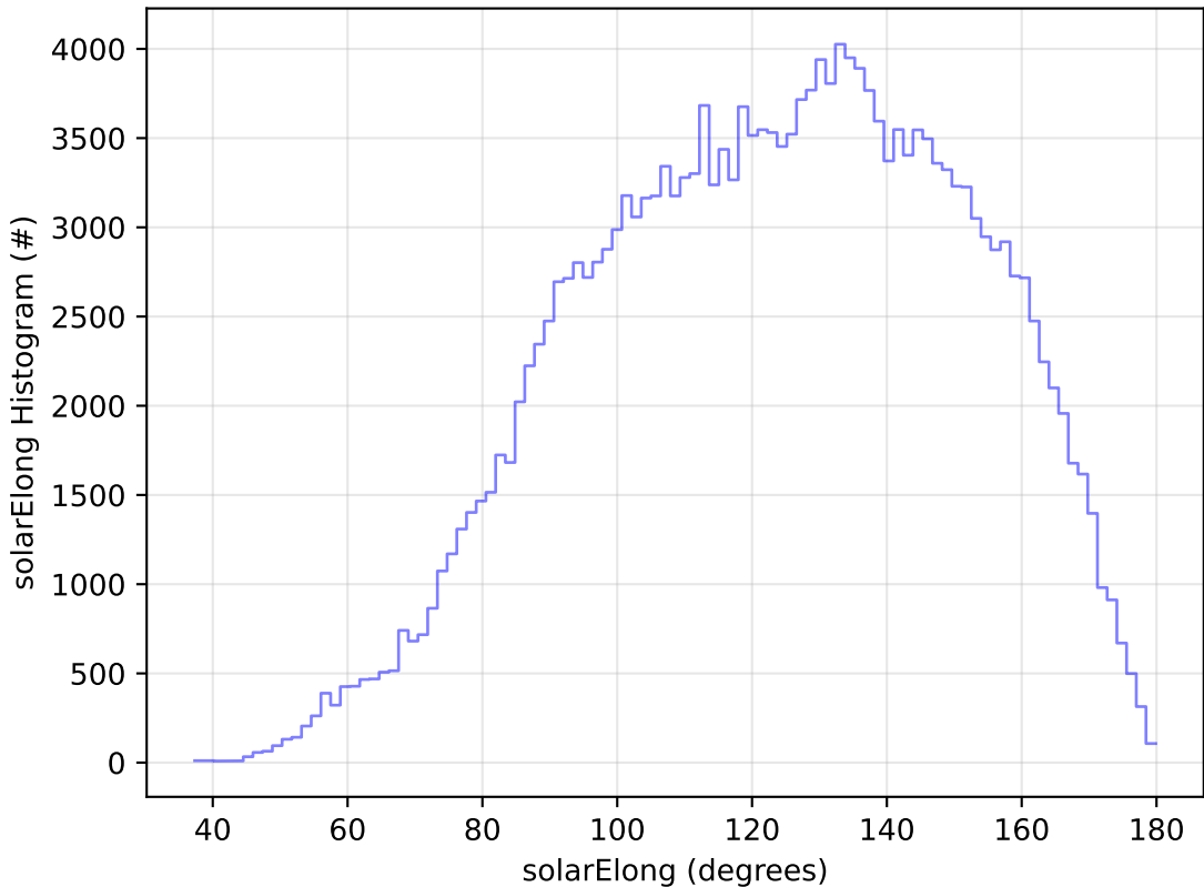
too_elab_r256_d3_griz_v3.4_10yrs WFD g band: solarElong Histogram
