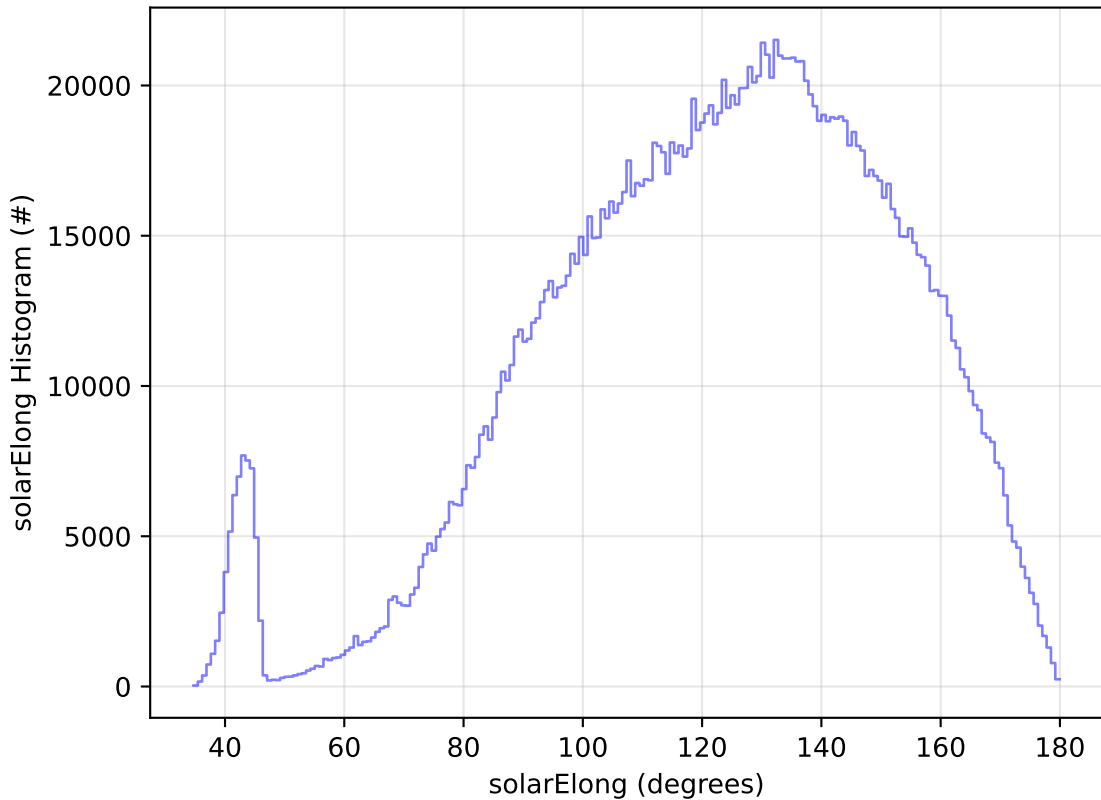
too_elab_r256_d3_griz_v3.4_10yrs WFD all bands: solarElong Histogram
