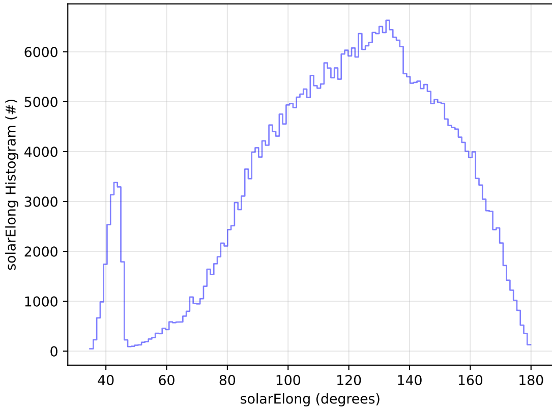
too_elab_r256_d3_griz_v3.4_10yrs All sky z band: solarElong Histogram
