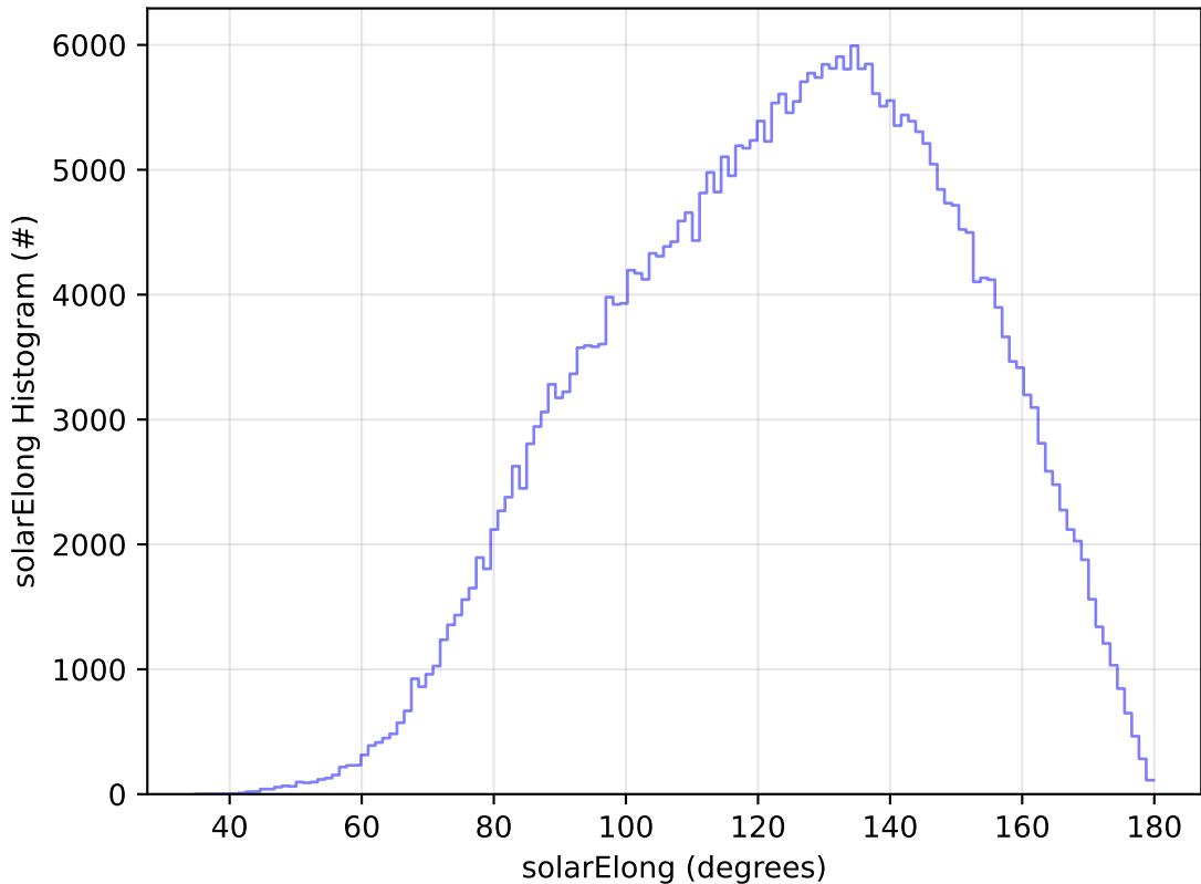
too_elab_r256_d3_griz_v3.4_10yrs All sky y band: solarElong Histogram
