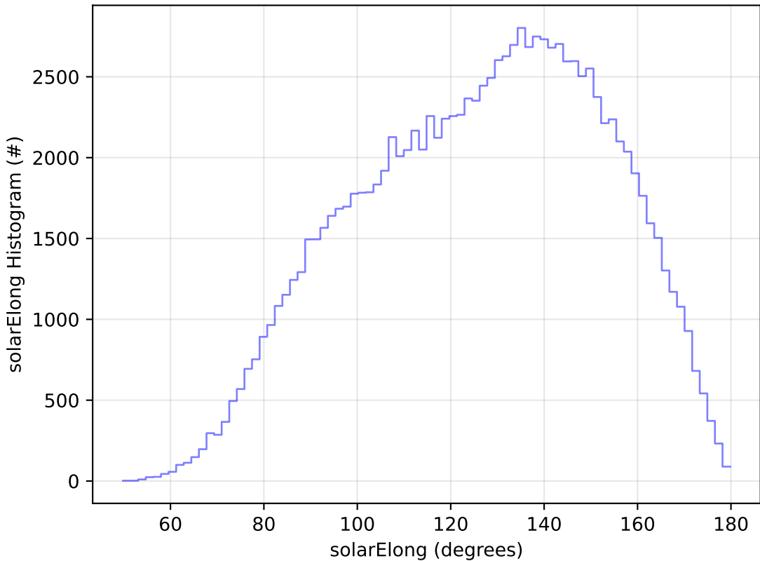
too_elab_r256_d3_griz_v3.4_10yrs All sky u band: solarElong Histogram
