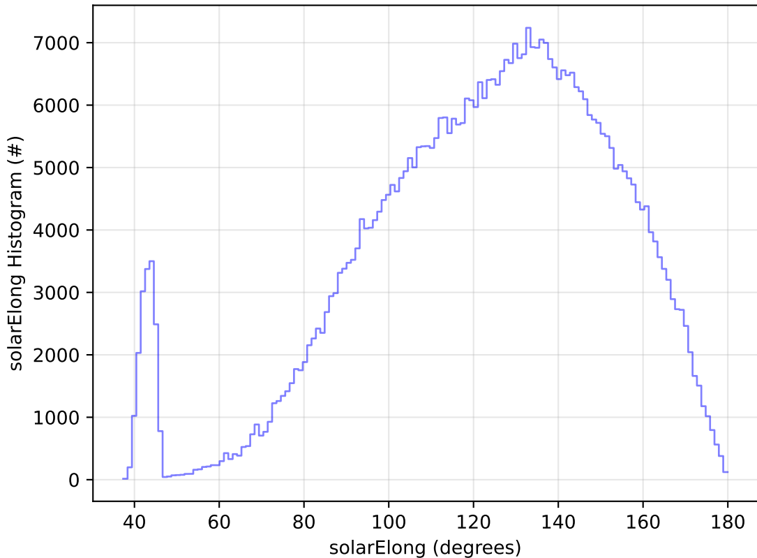
too_elab_r256_d3_griz_v3.4_10yrs All sky r band: solarElong Histogram
