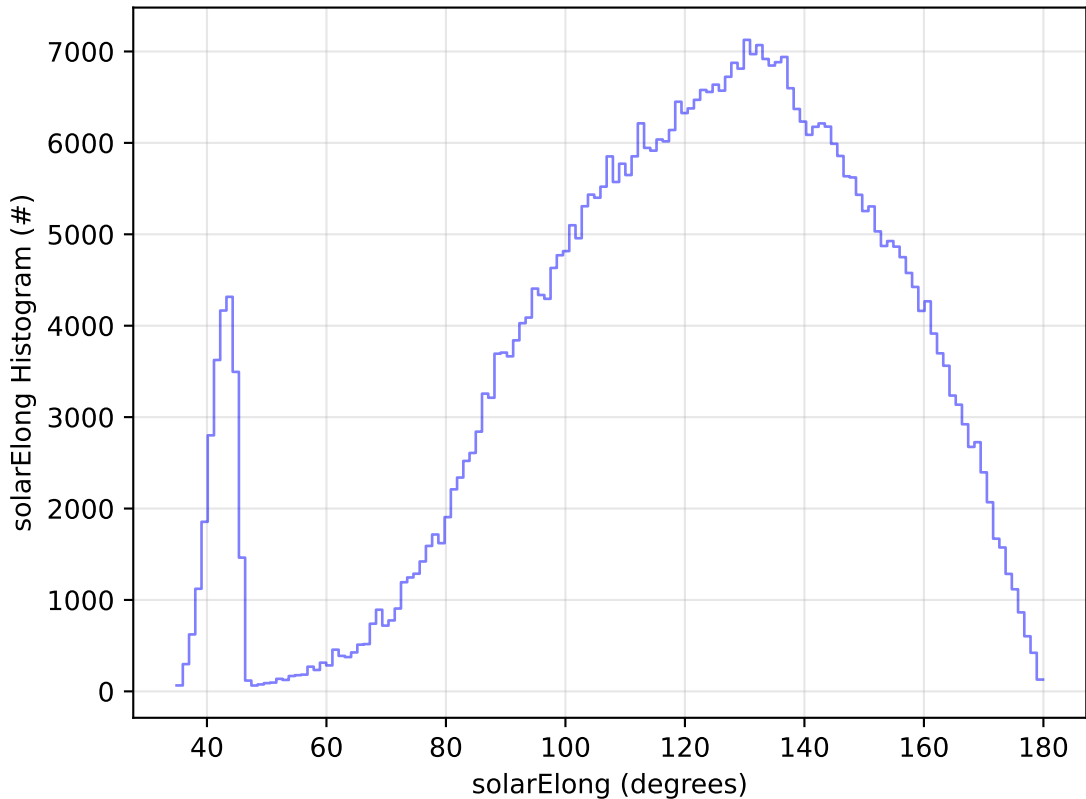
too_elab_r256_d3_griz_v3.4_10yrs All sky i band: solarElong Histogram
