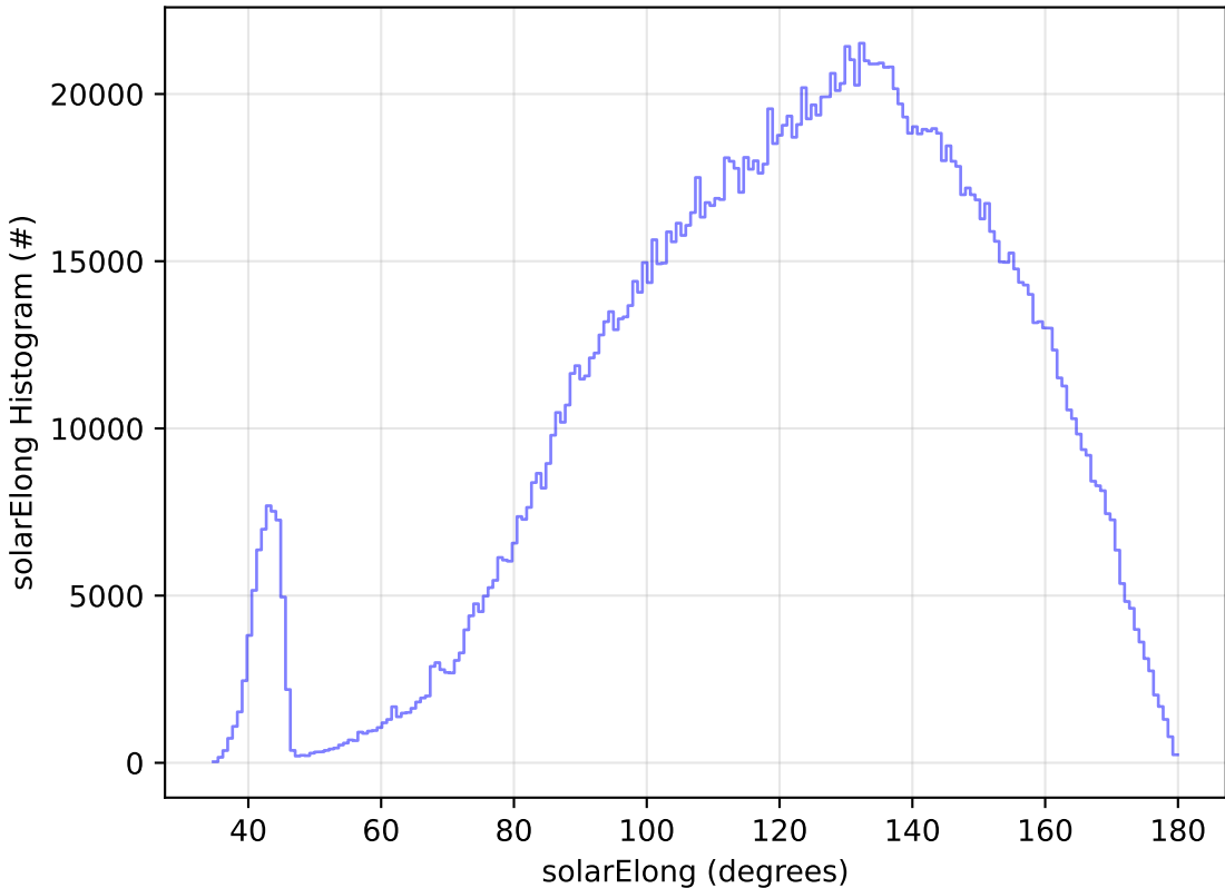
too_elab_r256_d3_griz_v3.4_10yrs All sky all bands: solarElong Histogram
