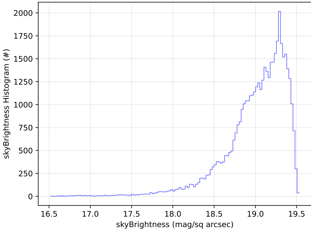
too_elab_r256_d3_griz_v3.4_10yrs Yr 1 z band: skyBrightness Histogram
