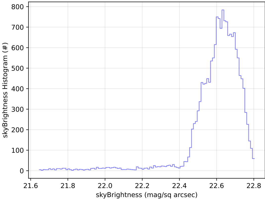
too_elab_r256_d3_griz_v3.4_10yrs Yr 1 u band: skyBrightness Histogram
