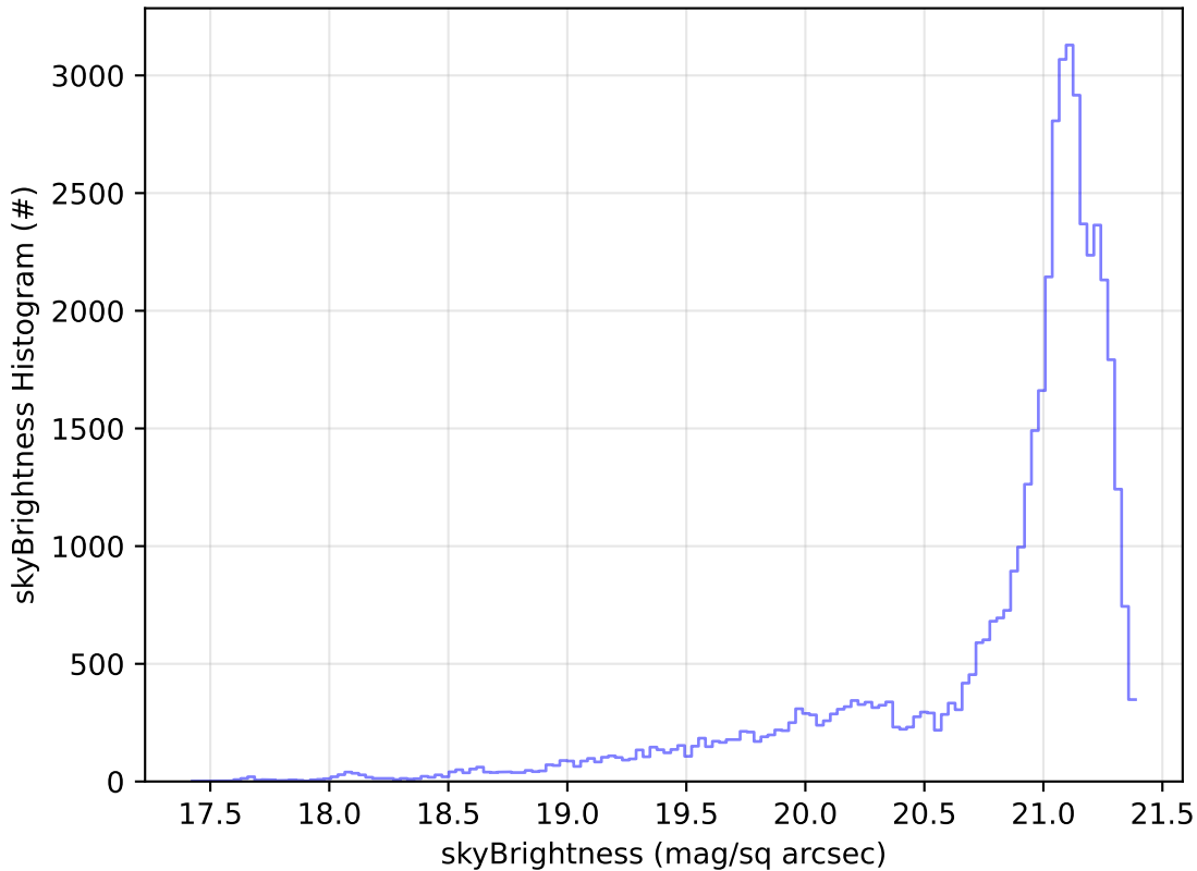
too_elab_r256_d3_griz_v3.4_10yrs Yr 1 r band: skyBrightness Histogram
