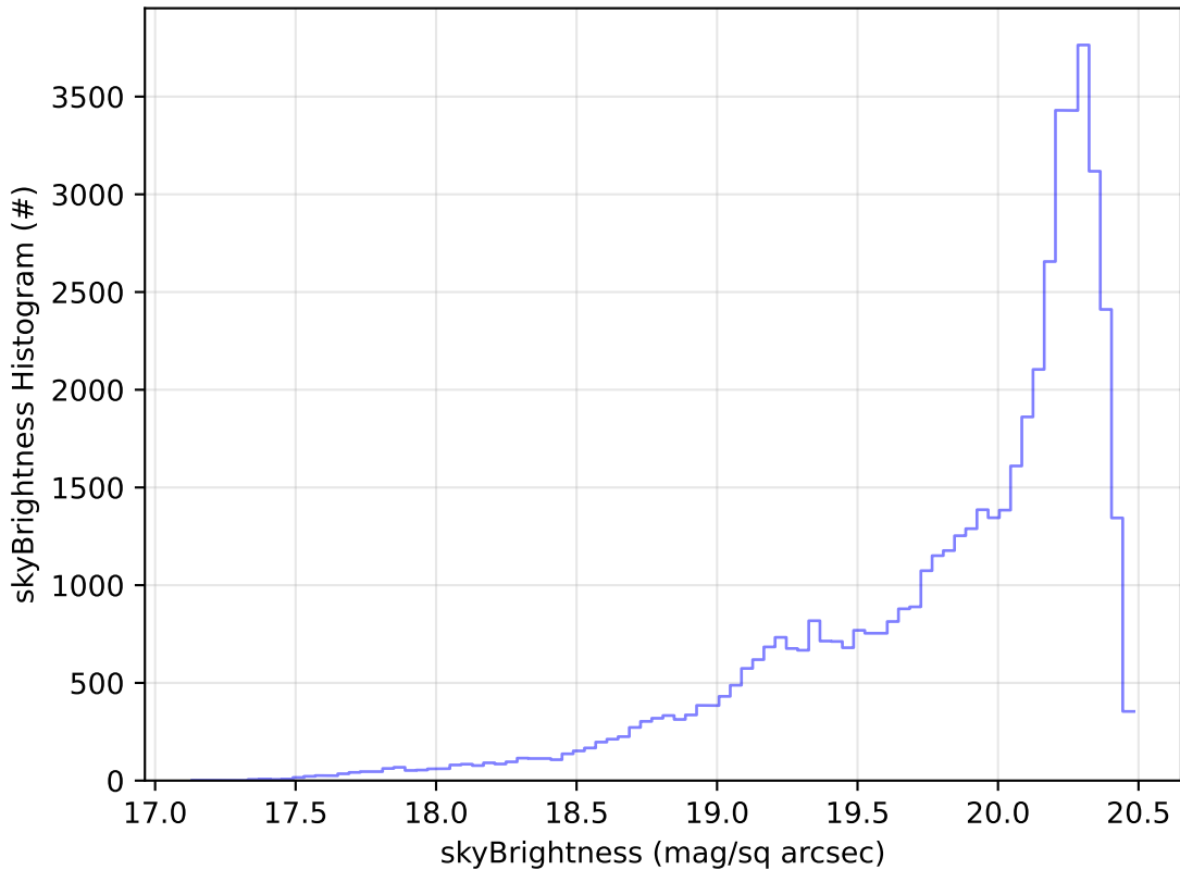
too_elab_r256_d3_griz_v3.4_10yrs Yr 1 i band: skyBrightness Histogram
