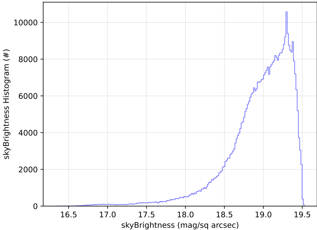
too_elab_r256_d3_griz_v3.4_10yrs WFD z band: skyBrightness Histogram
