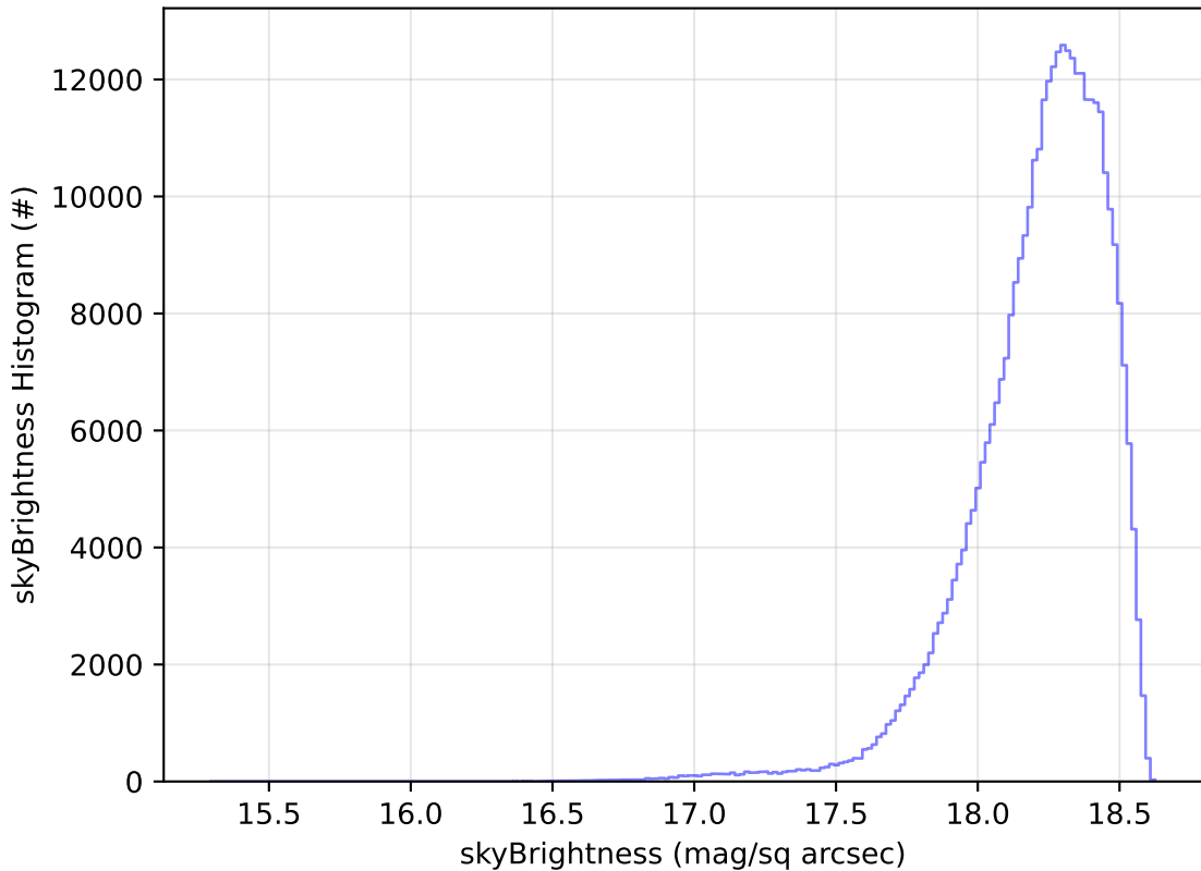
too_elab_r256_d3_griz_v3.4_10yrs WFD y band: skyBrightness Histogram
