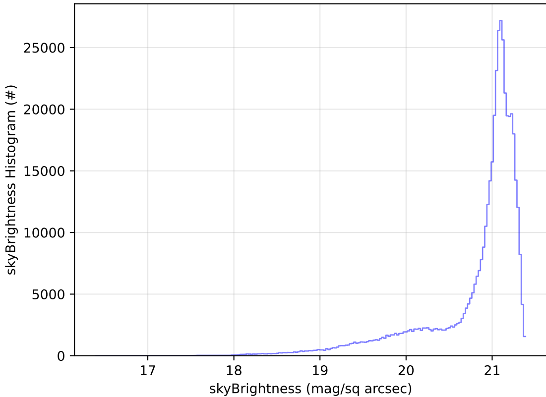
too_elab_r256_d3_griz_v3.4_10yrs WFD r band: skyBrightness Histogram
