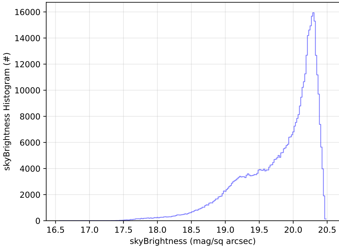
too_elab_r256_d3_griz_v3.4_10yrs WFD i band: skyBrightness Histogram
