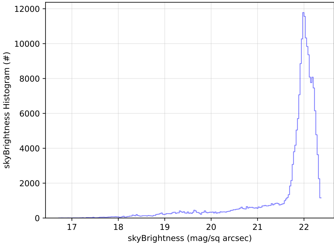
too_elab_r256_d3_griz_v3.4_10yrs WFD g band: skyBrightness Histogram
