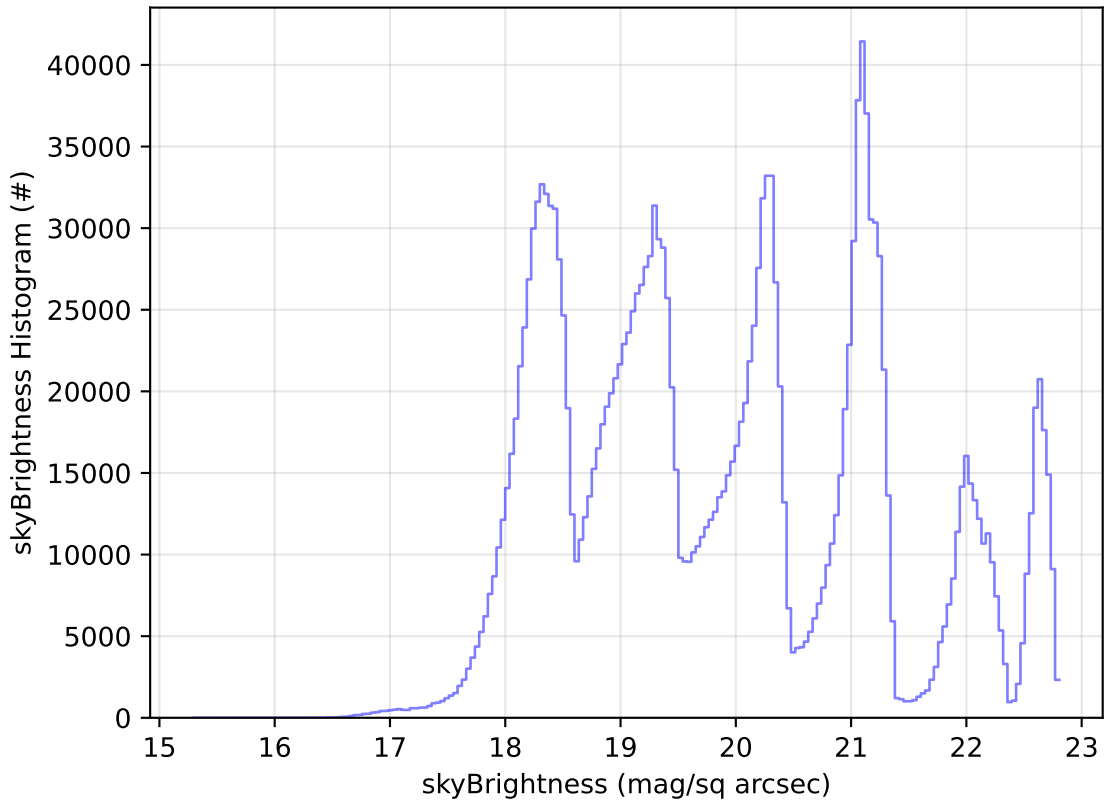
too_elab_r256_d3_griz_v3.4_10yrs WFD all bands: skyBrightness Histogram
