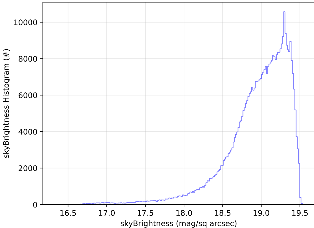
too_elab_r256_d3_griz_v3.4_10yrs All sky z band: skyBrightness Histogram
