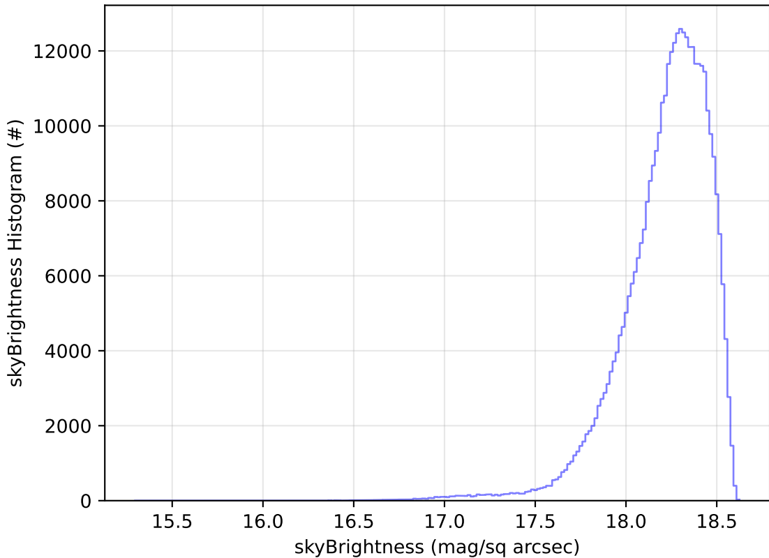
too_elab_r256_d3_griz_v3.4_10yrs All sky y band: skyBrightness Histogram
