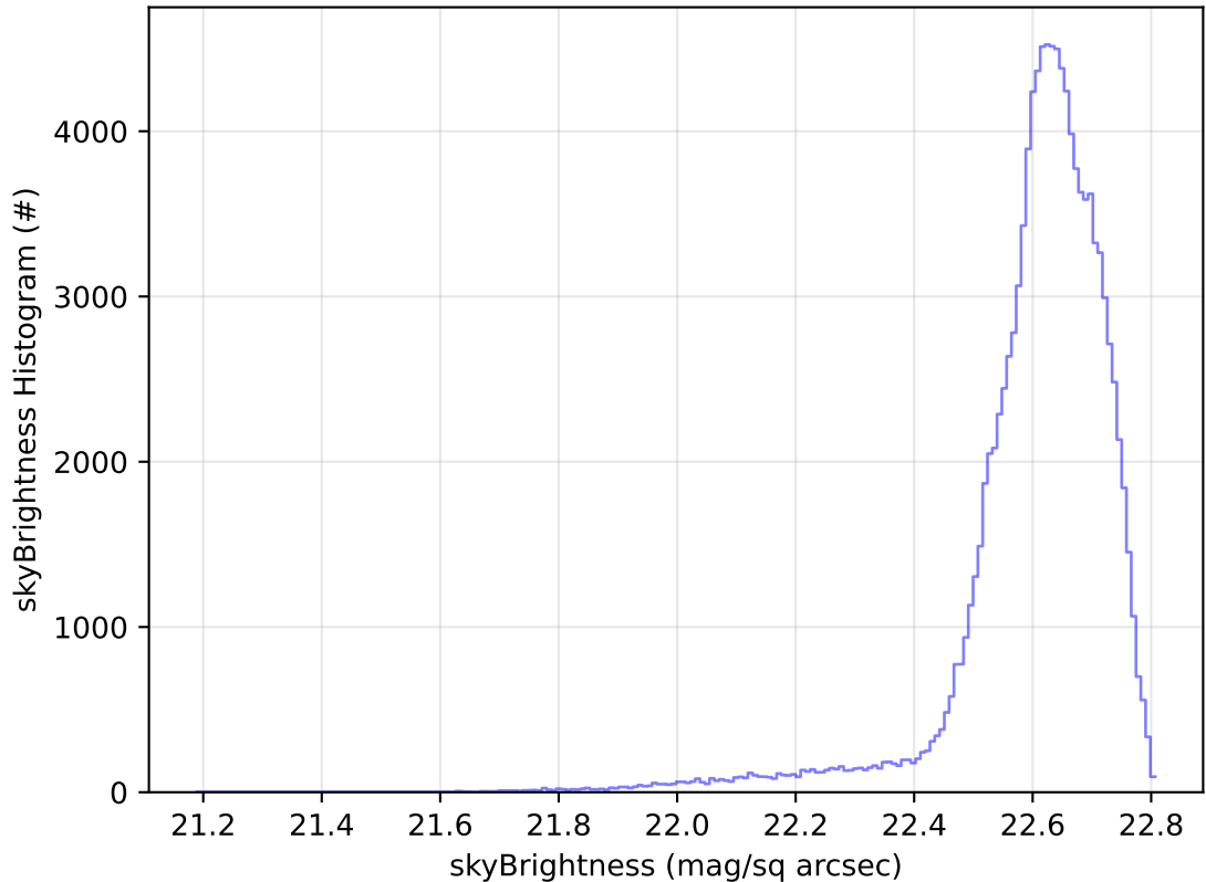
too_elab_r256_d3_griz_v3.4_10yrs All sky u band: skyBrightness Histogram
