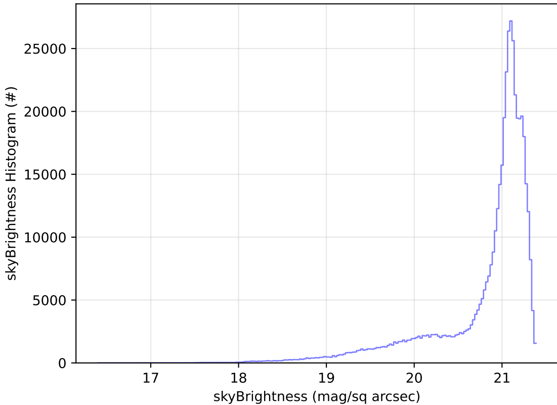
too_elab_r256_d3_griz_v3.4_10yrs All sky r band: skyBrightness Histogram
