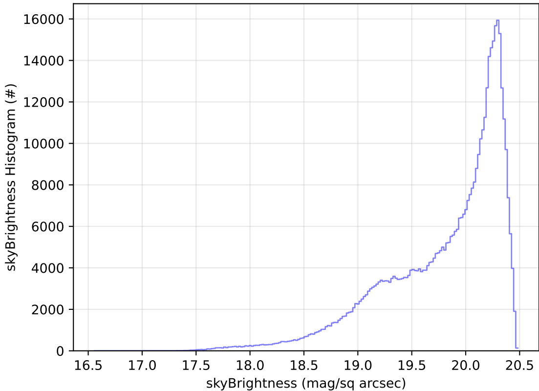
too_elab_r256_d3_griz_v3.4_10yrs All sky i band: skyBrightness Histogram
