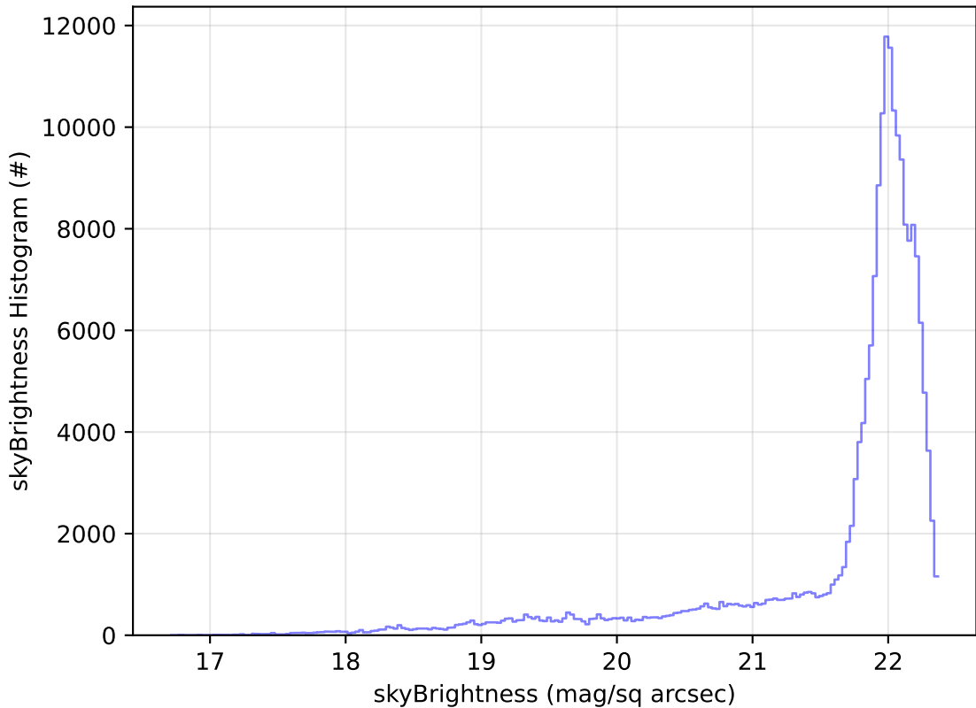
too_elab_r256_d3_griz_v3.4_10yrs All sky g band: skyBrightness Histogram
