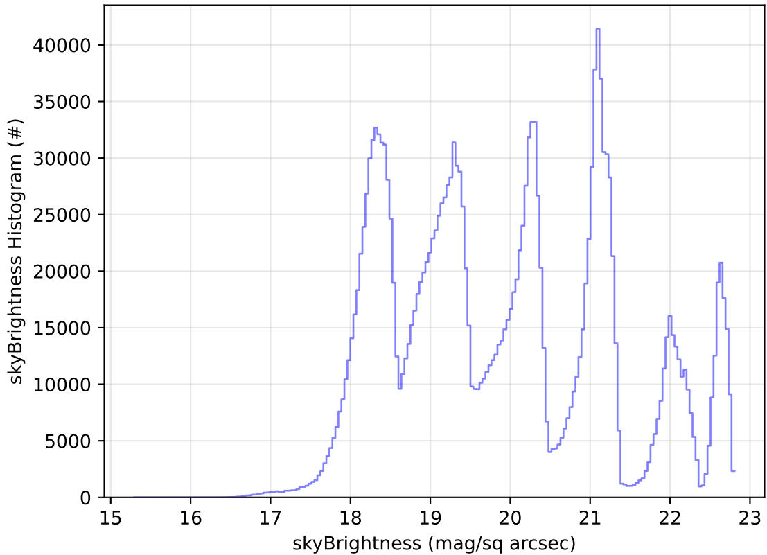
too_elab_r256_d3_griz_v3.4_10yrs All sky all bands: skyBrightness Histogram
