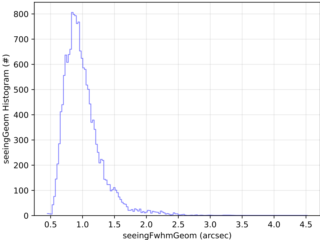
too_elab_r256_d3_griz_v3.4_10yrs Yr 1 u band: seeingGeom Histogram
