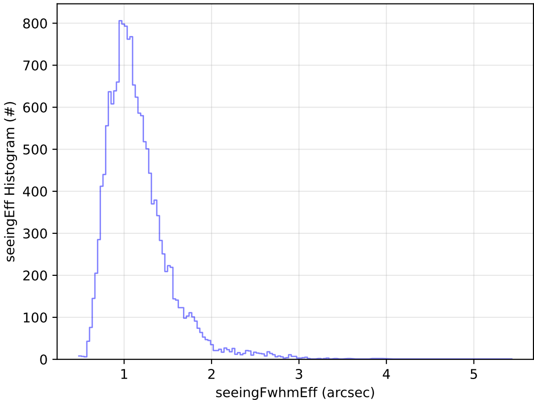
too_elab_r256_d3_griz_v3.4_10yrs Yr 1 u band: seeingEff Histogram
