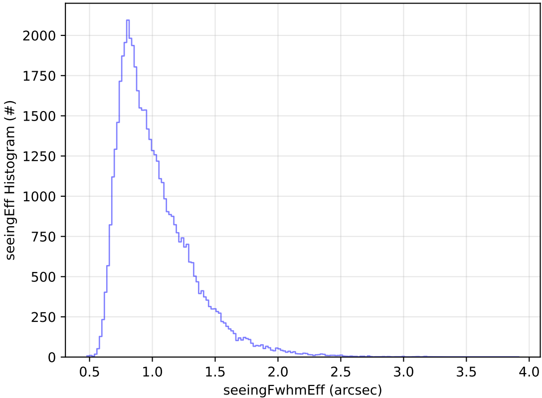
too_elab_r256_d3_griz_v3.4_10yrs Yr 1 r band: seeingEff Histogram
