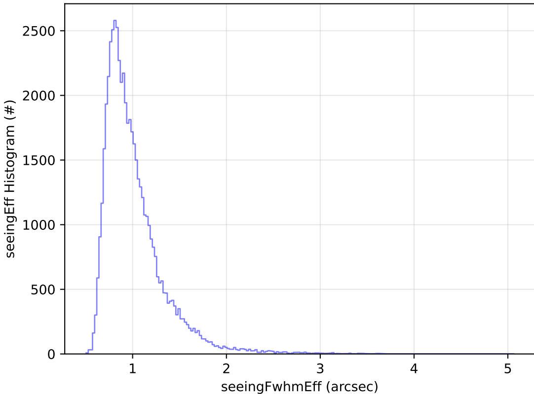
too_elab_r256_d3_griz_v3.4_10yrs Yr 1 i band: seeingEff Histogram
