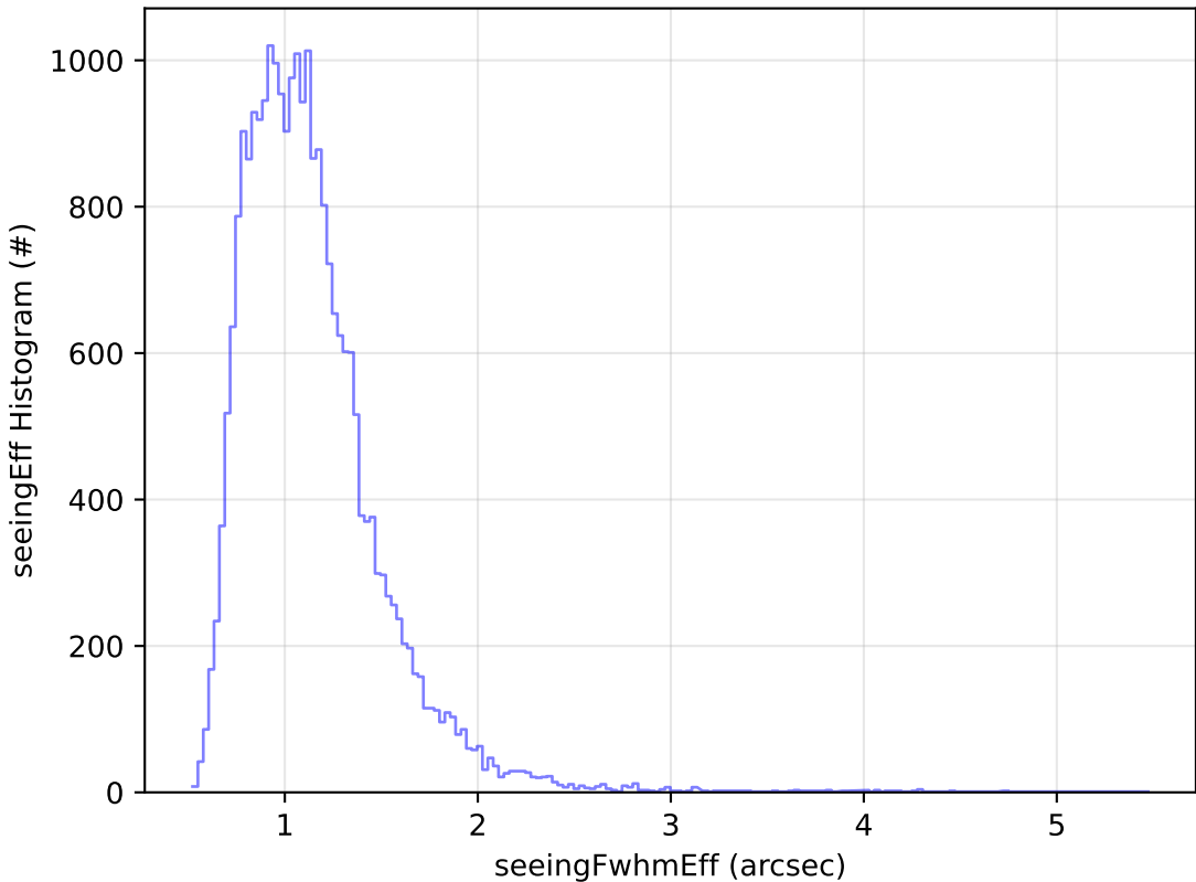
too_elab_r256_d3_griz_v3.4_10yrs Yr 1 g band: seeingEff Histogram
