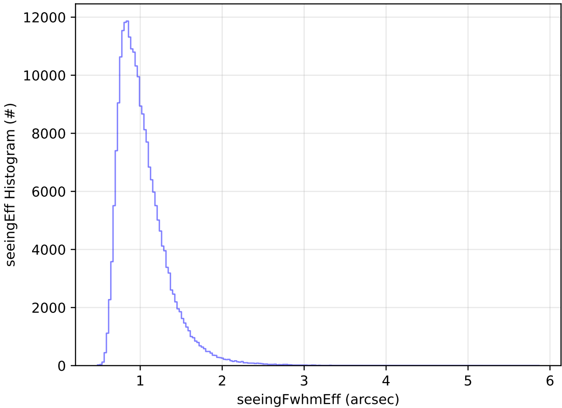
too_elab_r256_d3_griz_v3.4_10yrs Yr 1 all bands: seeingEff Histogram
