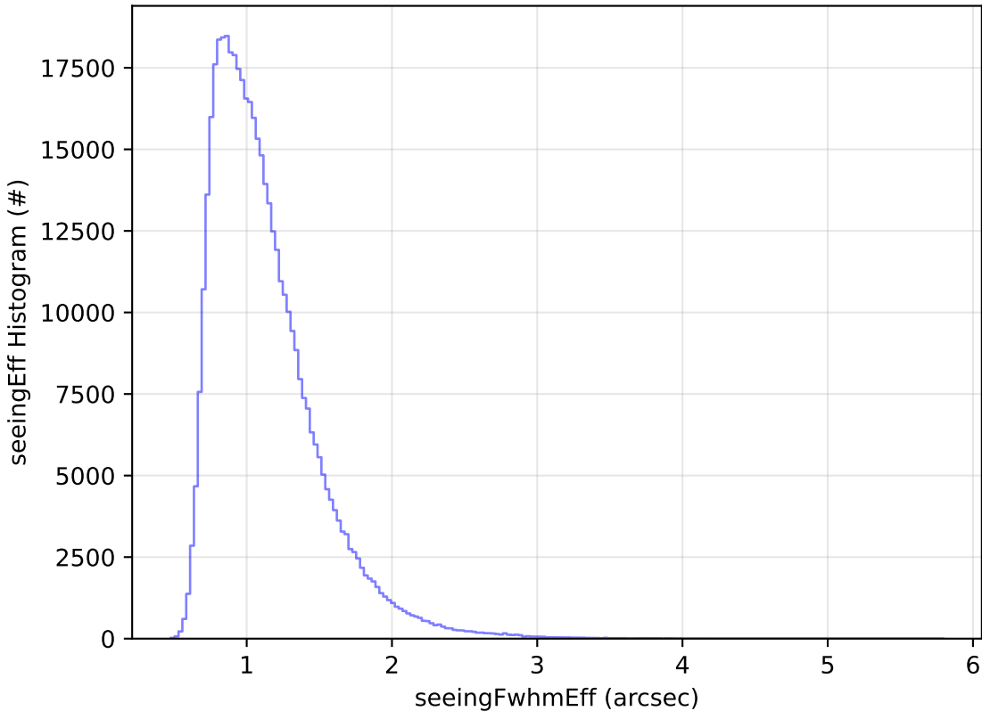
too_elab_r256_d3_griz_v3.4_10yrs WFD r band: seeingEff Histogram
