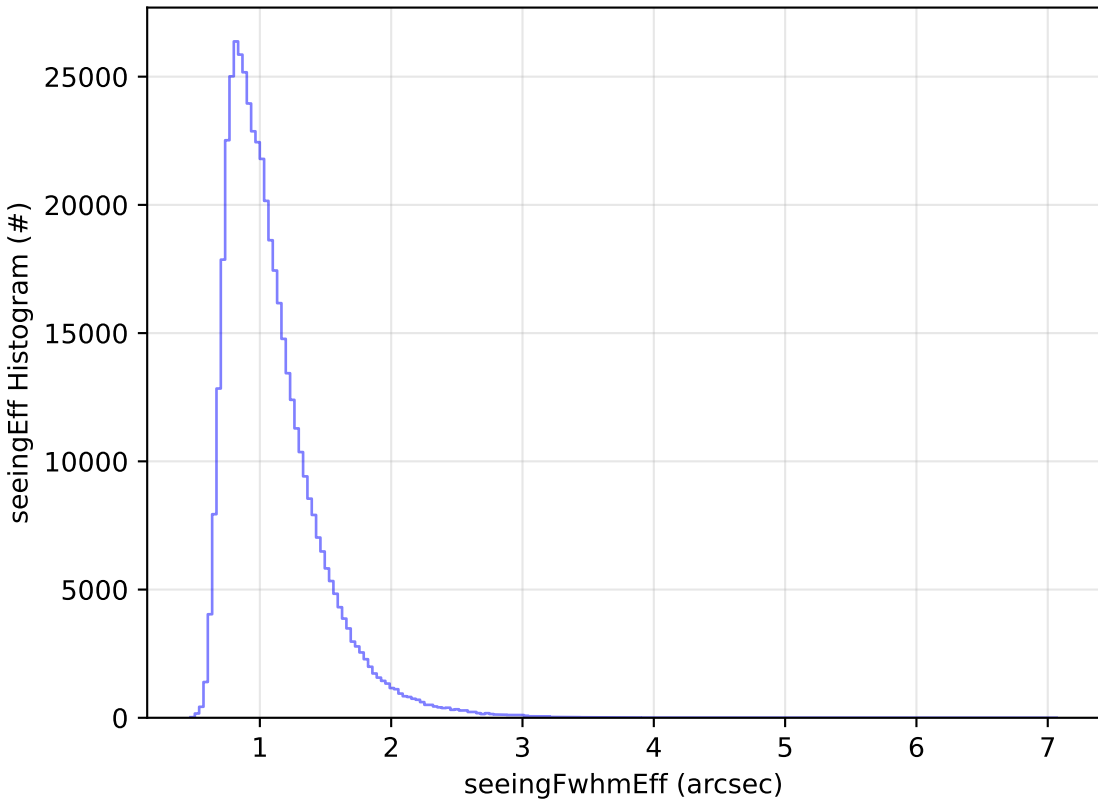
too_elab_r256_d3_griz_v3.4_10yrs WFD i band: seeingEff Histogram
