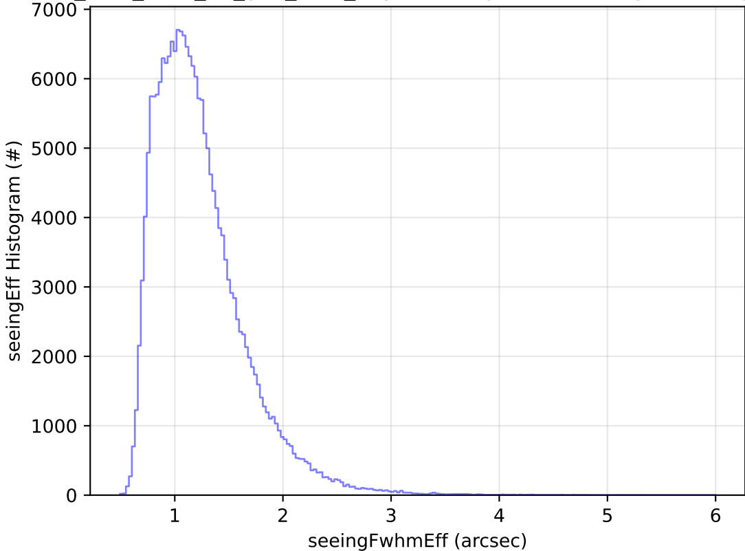
too_elab_r256_d3_griz_v3.4_10yrs WFD g band: seeingEff Histogram
