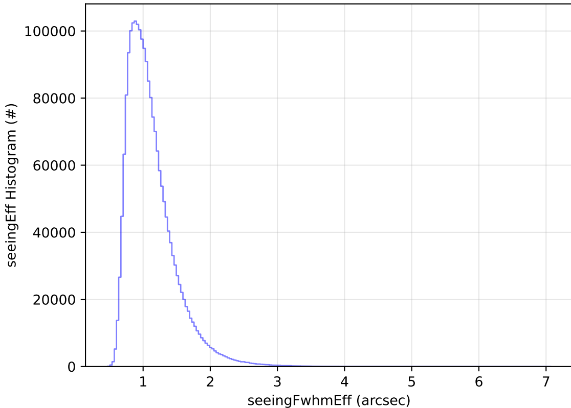
too_elab_r256_d3_griz_v3.4_10yrs WFD all bands: seeingEff Histogram
