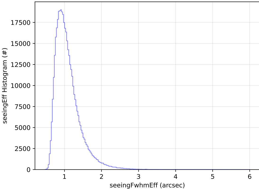
too_elab_r256_d3_griz_v3.4_10yrs All sky z band: seeingEff Histogram
