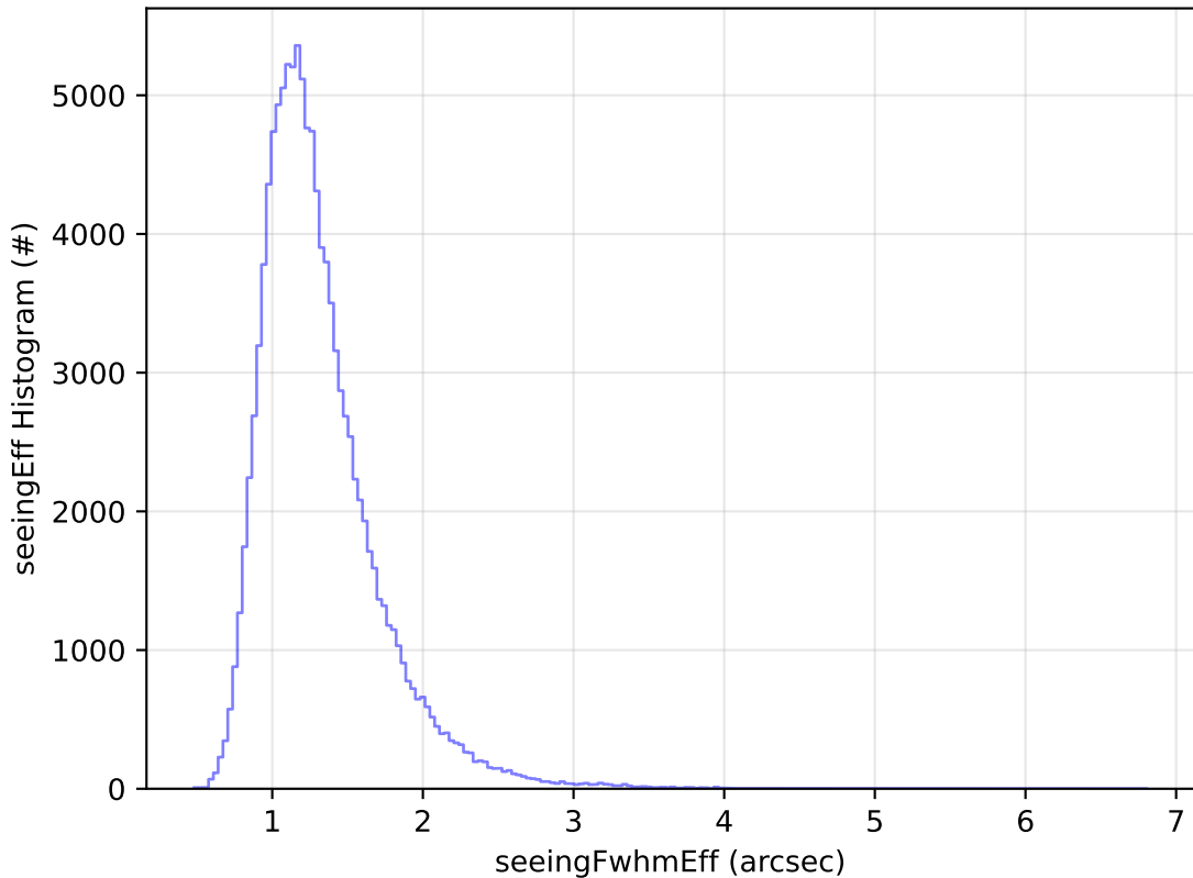
too_elab_r256_d3_griz_v3.4_10yrs All sky u band: seeingEff Histogram
