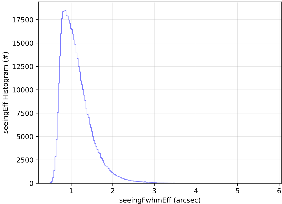
too_elab_r256_d3_griz_v3.4_10yrs All sky r band: seeingEff Histogram
