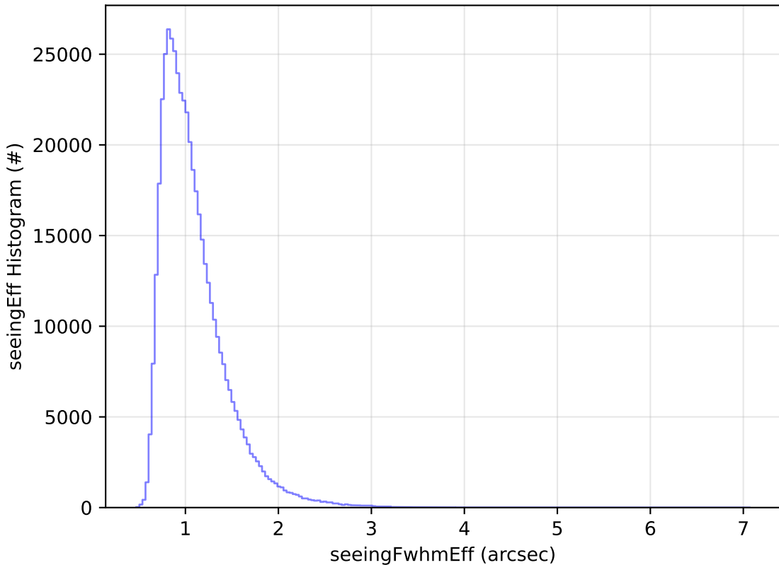
too_elab_r256_d3_griz_v3.4_10yrs All sky i band: seeingEff Histogram
