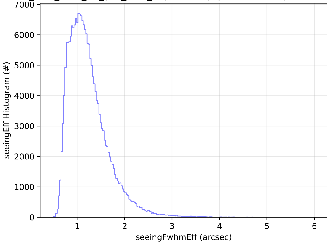
too_elab_r256_d3_griz_v3.4_10yrs All sky g band: seeingEff Histogram
