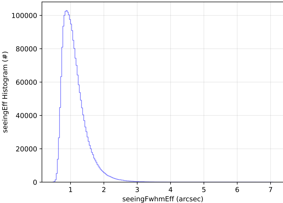
too_elab_r256_d3_griz_v3.4_10yrs All sky all bands: seeingEff Histogram
