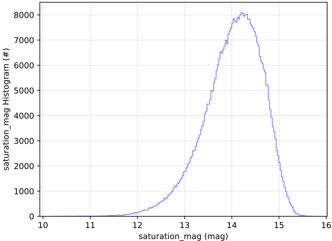
too_elab_r256_d3_griz_v3.4_10yrs WFD z band: saturation_mag Histogram
